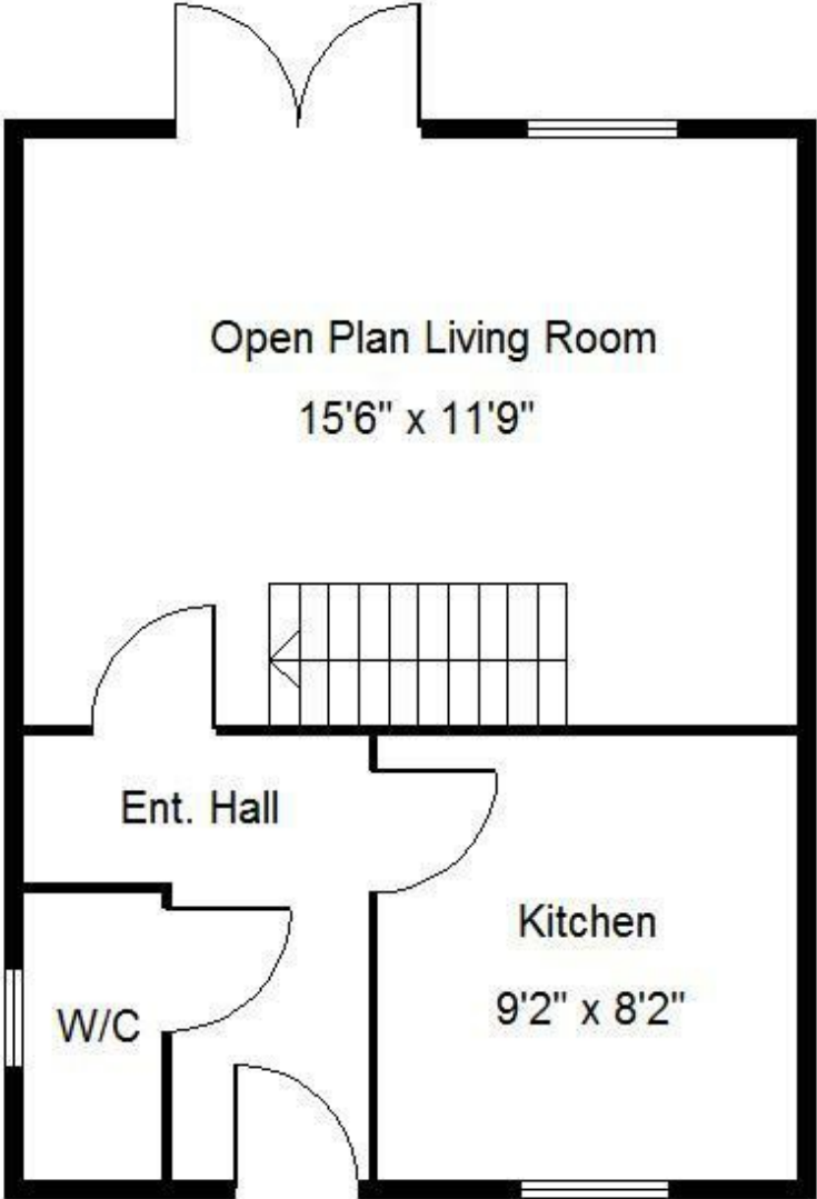
Ground Floor
