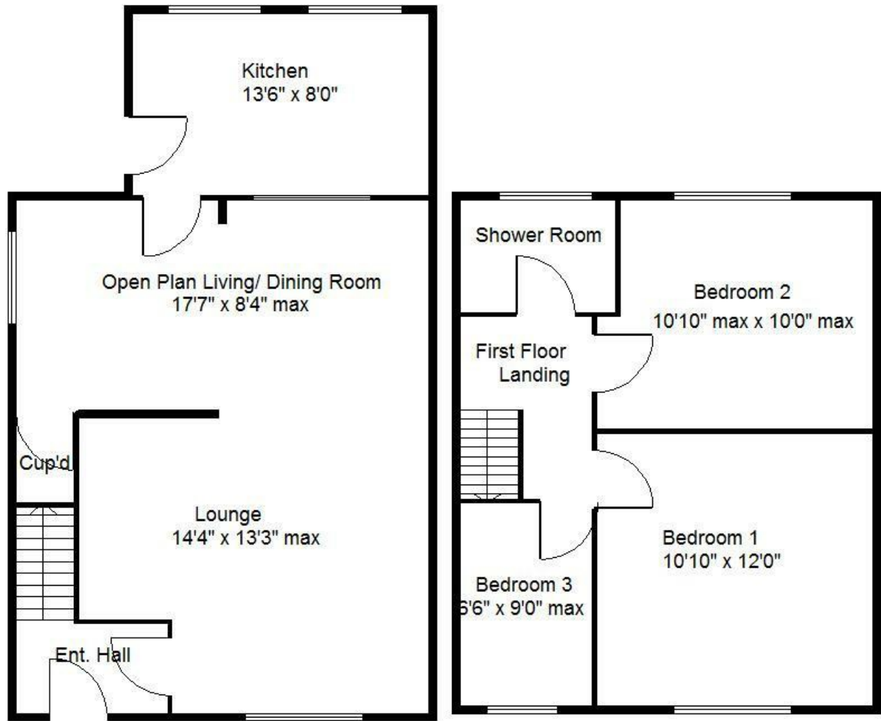
First Floor
